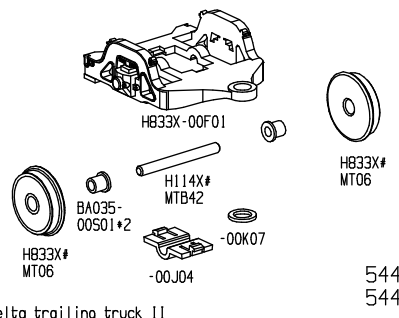
Delta trailing truck II
