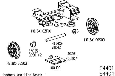
Hodges trailing truck I
