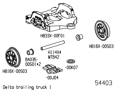
Delta trailing truck I
